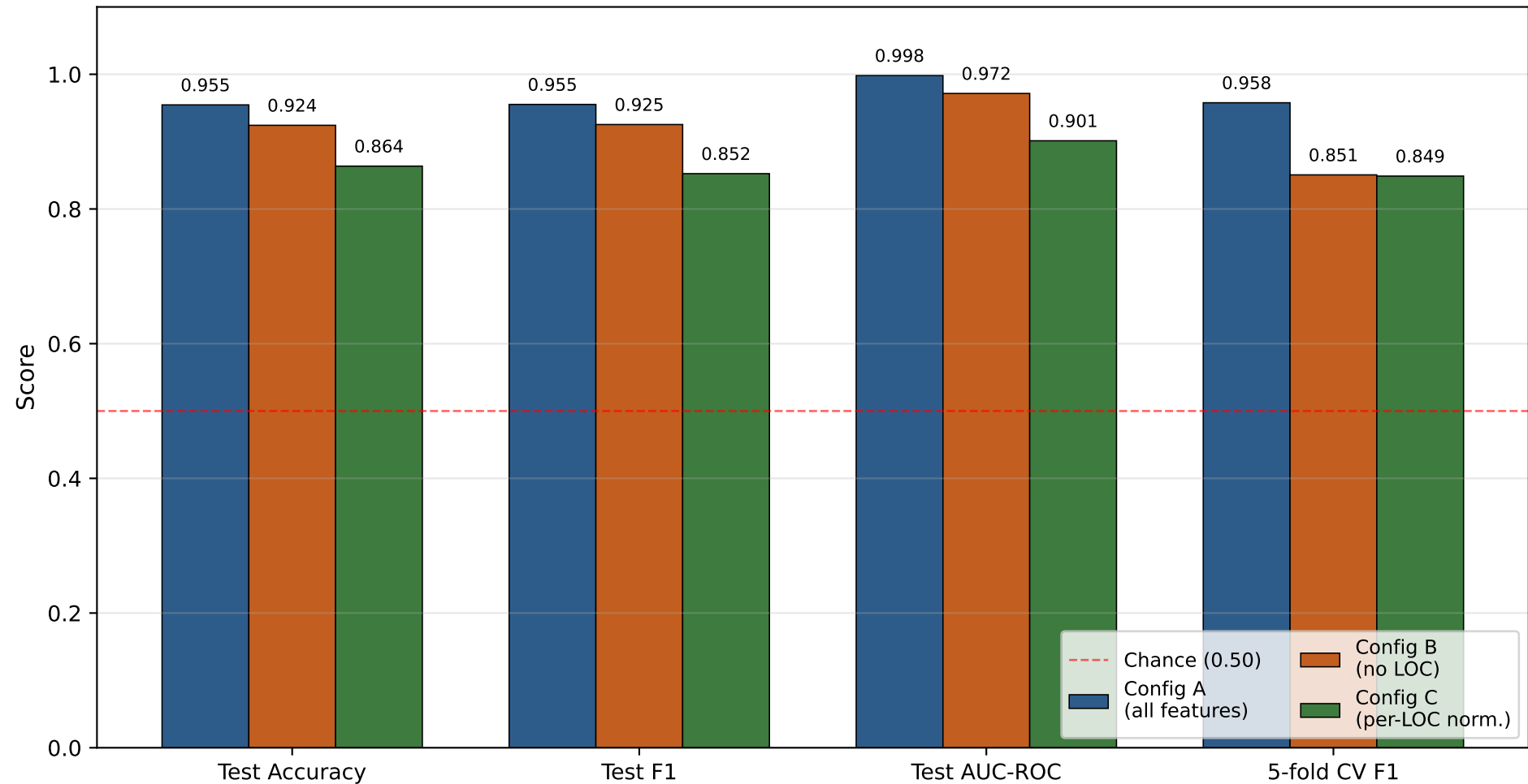
RQ7: Classification performance across configurations
